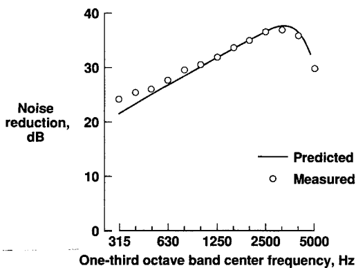
Fig. 3 Measured and VAPEPS predicted noise reduction of a 57.5 × 45.5 × 0.25-in. acrylic plate.
