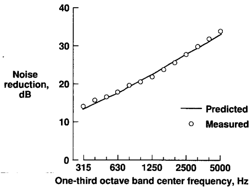
Fig. 2 Measured and VAPEPS predicted noise reduction of a 57.5 × 45.5 × 0.032-in. aluminum plate.
