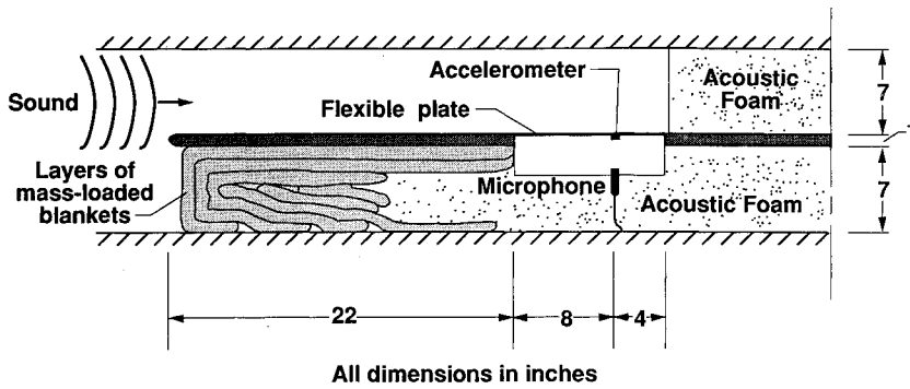
Fig. 5 Test configuration of a 12 × 8 × 0.040-in. aluminum plate subjected to broadband acoustic excitation in a wind tunnel with no flow.
