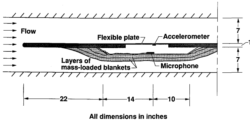
Fig. 9 Wind-tunnel test configuration of a 12 × 8 × 0.040-in. aluminum plate subjected to boundary-layer excitation.
