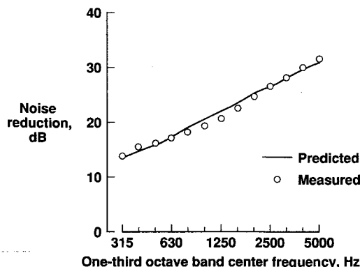
Fig. 4 Measured and VAPEPS predicted noise reduction of a 57.5 × 33.5 × 0.045-in. graphite-epoxy plate.
