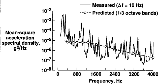
Fig. 11 Measured and VAPEPS predicted mean-square acceleration spectral density of the plate vibration in the wind tunnel due to turbulent boundary-layer excitation ( U = 90 ft/s).
